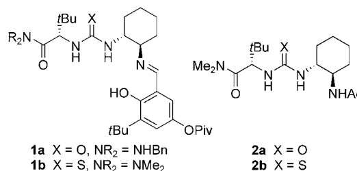
Figure 1. Urea and thiourea catalysts. Piv = pivaloyl.
